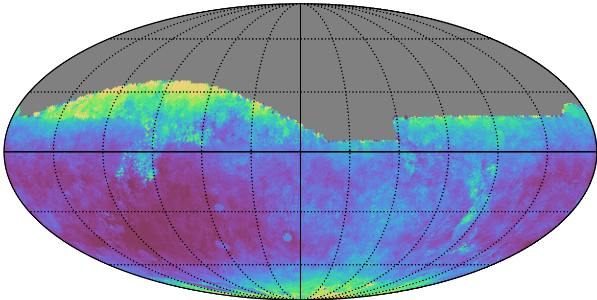
noroll_mjdp270_v3.4_10yrs All sky z band: Median seeingEff
