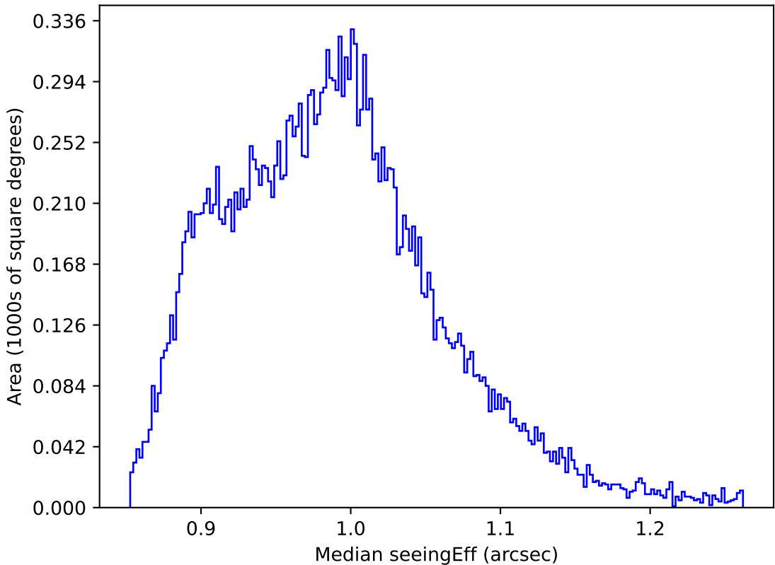
noroll_mjdp270_v3.4_10yrs All sky y band: Median seeingEff
