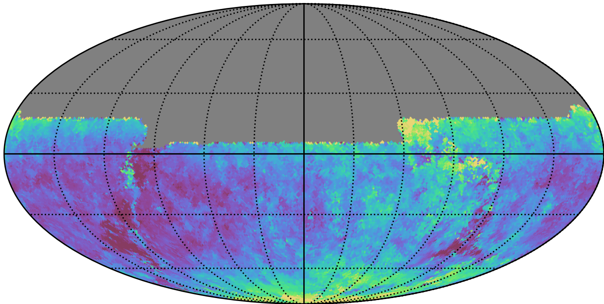
noroll_mjdp270_v3.4_10yrs All sky u band: Median seeingEff
