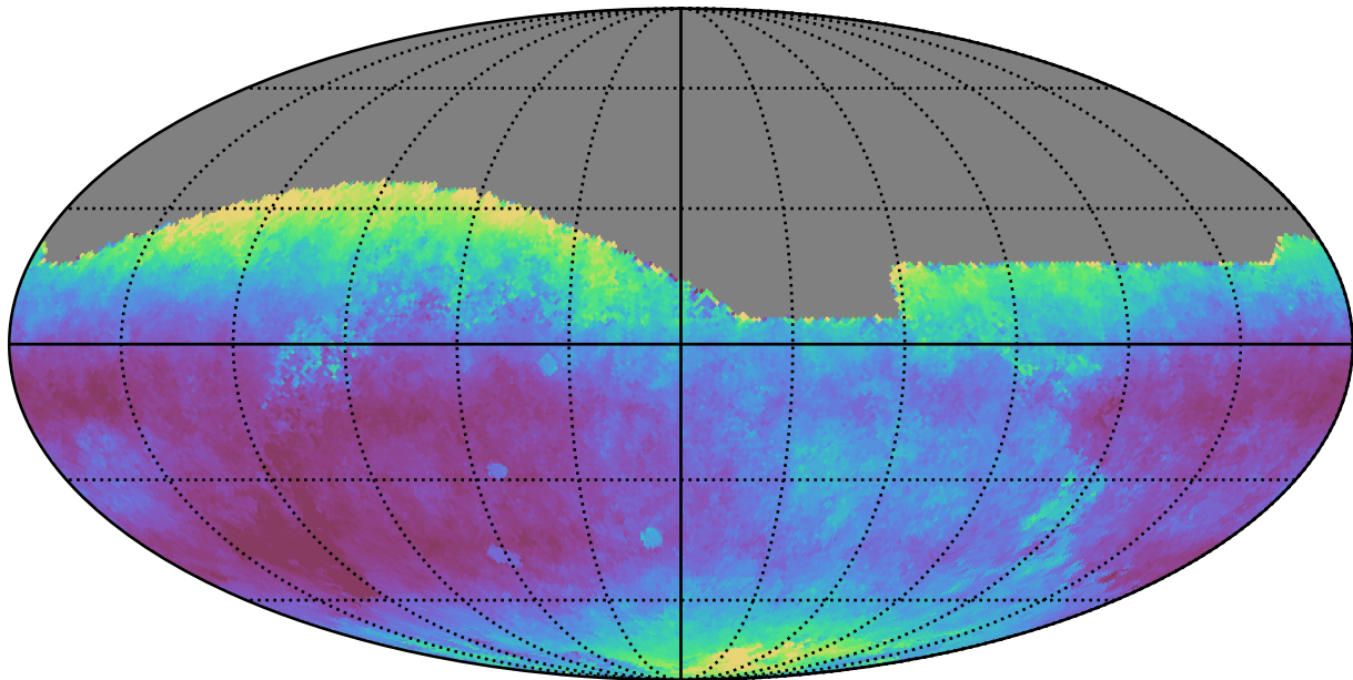
noroll_mjdp270_v3.4_10yrs All sky r band: Median seeingEff
