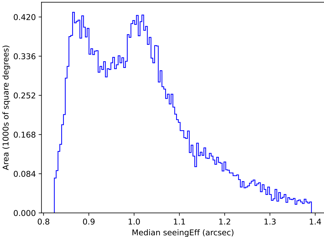
noroll_mjdp270_v3.4_10yrs All sky i band: Median seeingEff
