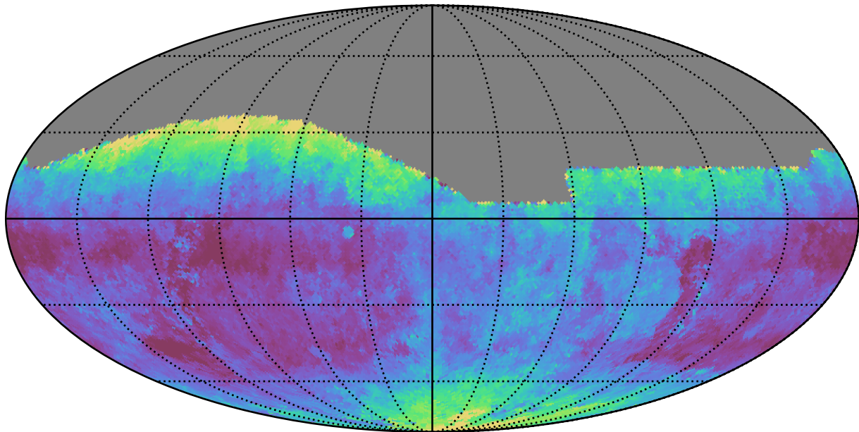
noroll_mjdp270_v3.4_10yrs All sky g band: Median seeingEff
