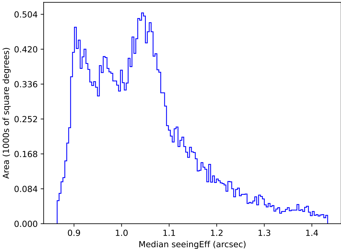
noroll_mjdp270_v3.4_10yrs All sky all bands: Median seeingEff
