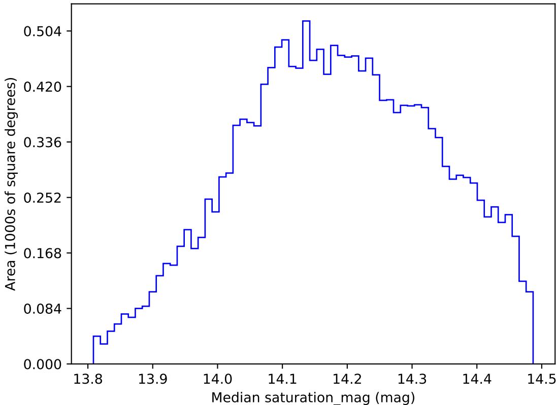
noroll_mjdp270_v3.4_10yrs WFD z band: Median saturation_mag
