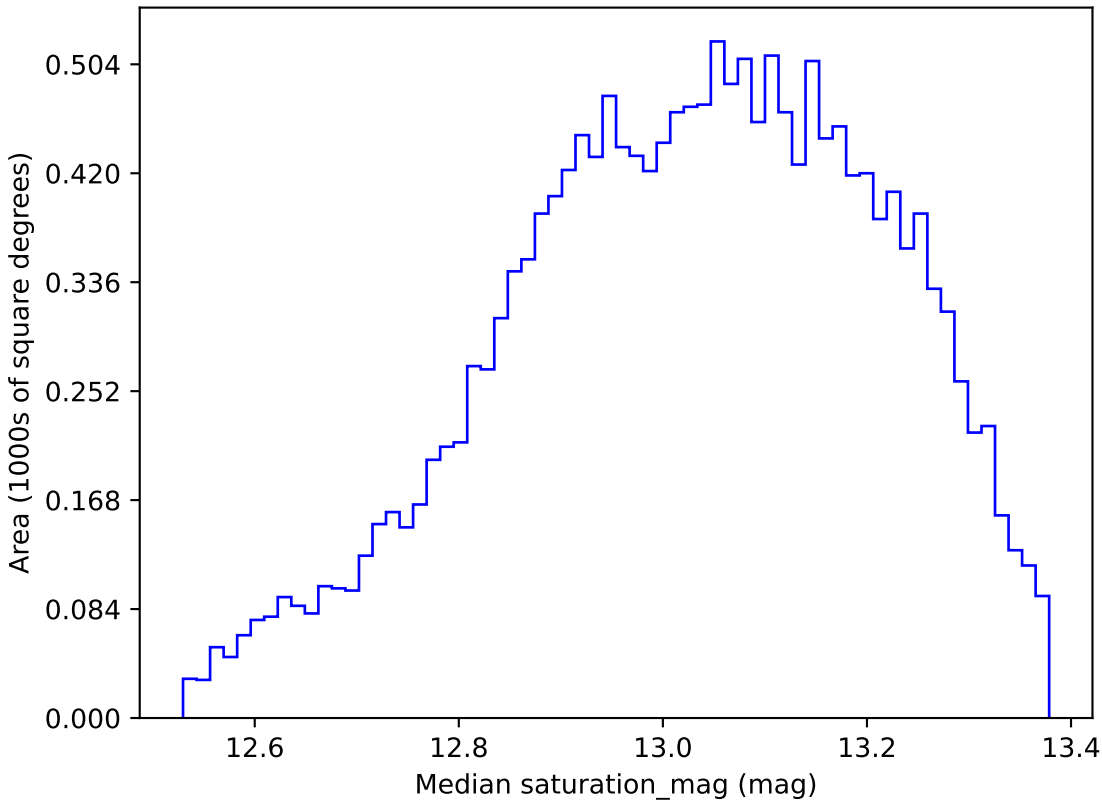
noroll_mjdp270_v3.4_10yrs WFD u band: Median saturation_mag
