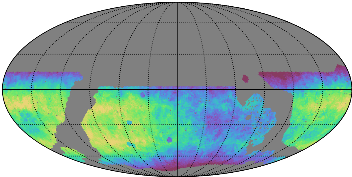
noroll_mjdp270_v3.4_10yrs WFD r band: Median saturation_mag
