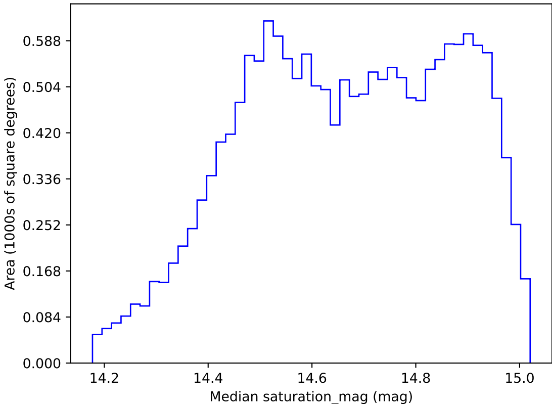
noroll_mjdp270_v3.4_10yrs WFD r band: Median saturation_mag
