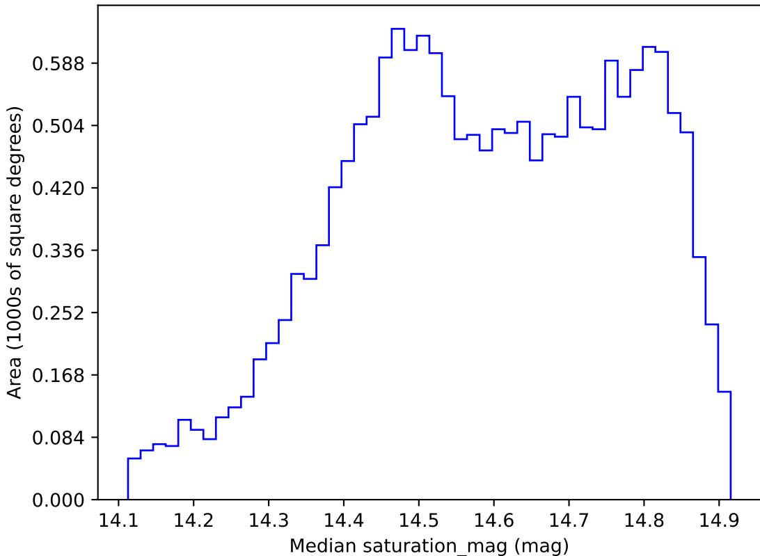
noroll_mjdp270_v3.4_10yrs WFD i band: Median saturation_mag
