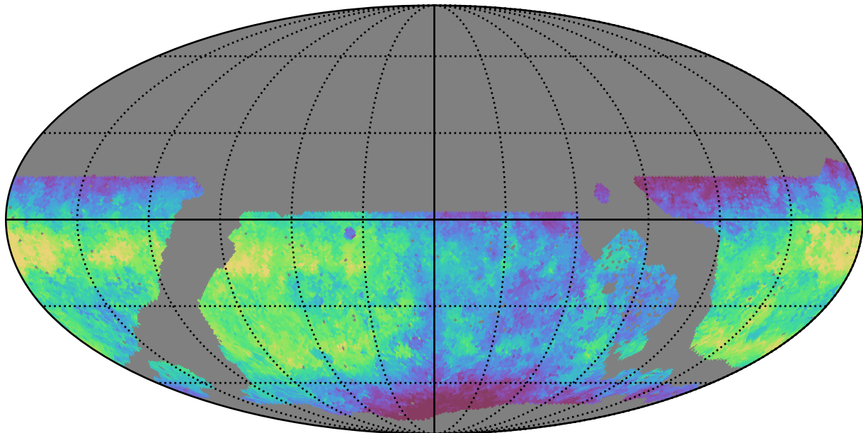
noroll_mjdp270_v3.4_10yrs WFD g band: Median saturation_mag
