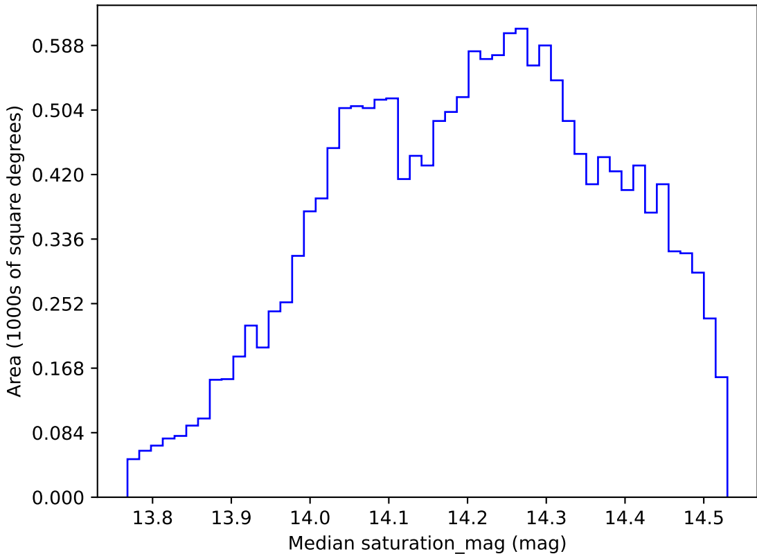
noroll_mjdp270_v3.4_10yrs WFD all bands: Median saturation_mag
