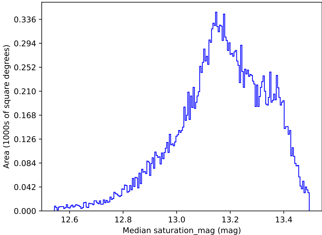
noroll_mjdp270_v3.4_10yrs All sky y band: Median saturation_mag
