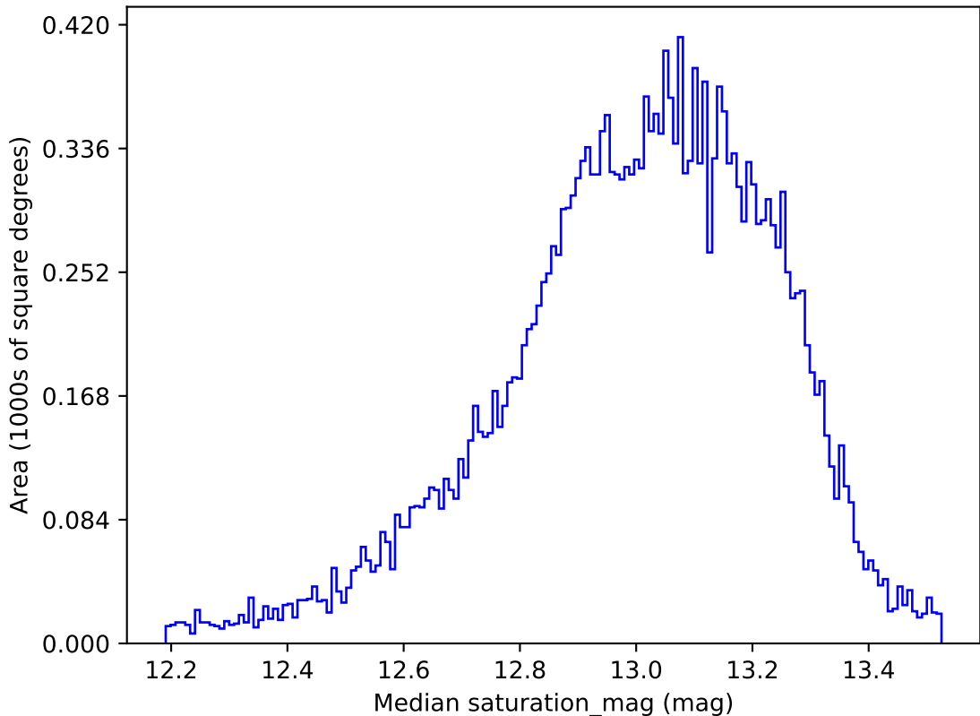
noroll_mjdp270_v3.4_10yrs All sky u band: Median saturation_mag
