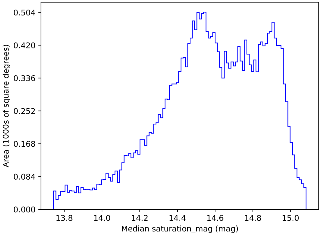
noroll_mjdp270_v3.4_10yrs All sky r band: Median saturation_mag
