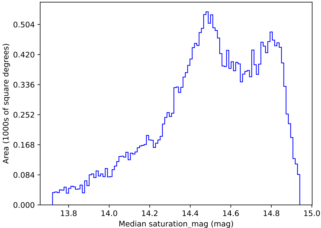
noroll_mjdp270_v3.4_10yrs All sky i band: Median saturation_mag
