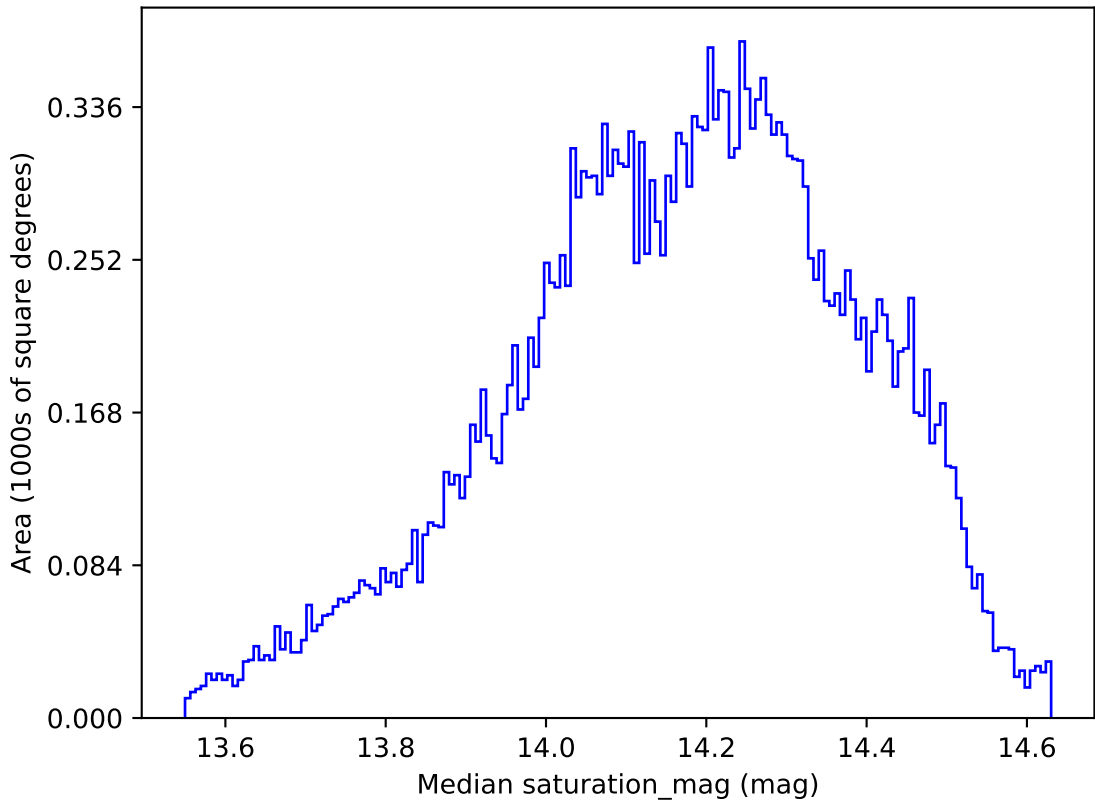
noroll_mjdp270_v3.4_10yrs All sky all bands: Median saturation_mag
