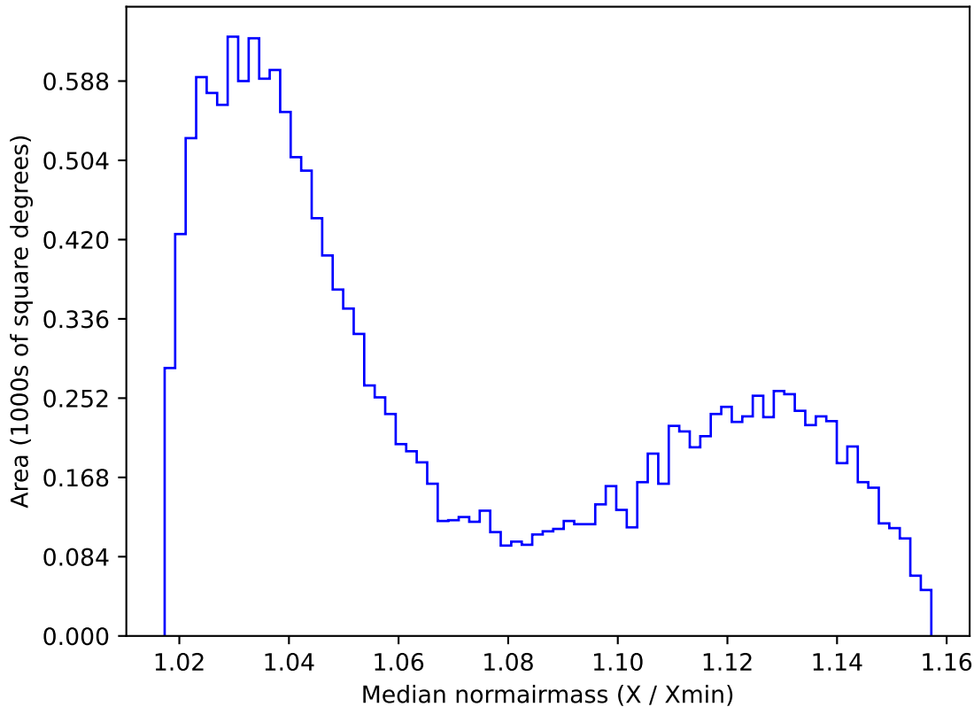
noroll_mjdp270_v3.4_10yrs WFD z band: Median normairmass
