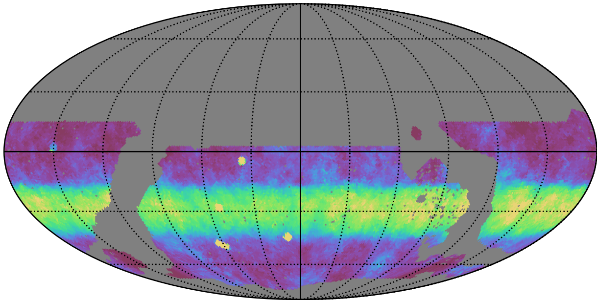
noroll_mjdp270_v3.4_10yrs WFD y band: Median normairmass
