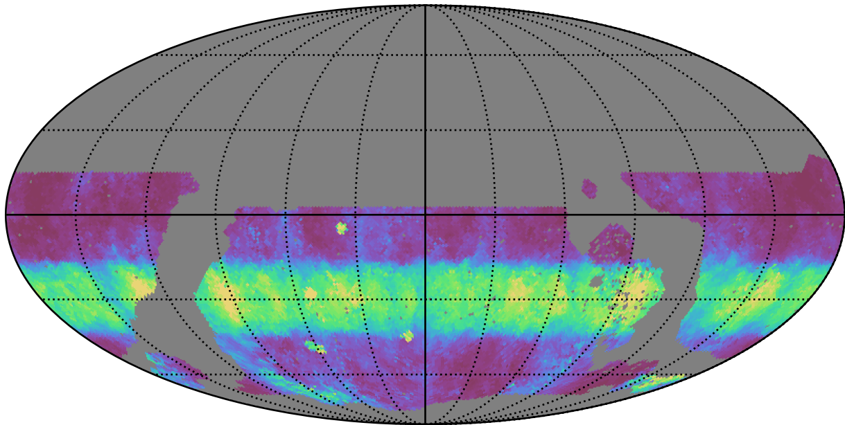
noroll_mjdp270_v3.4_10yrs WFD u band: Median normairmass
