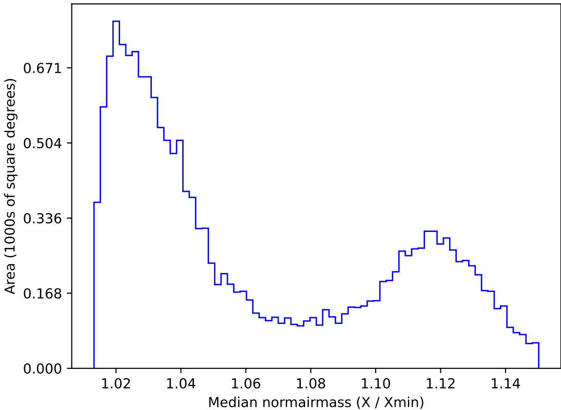
noroll_mjdp270_v3.4_10yrs WFD r band: Median normairmass
