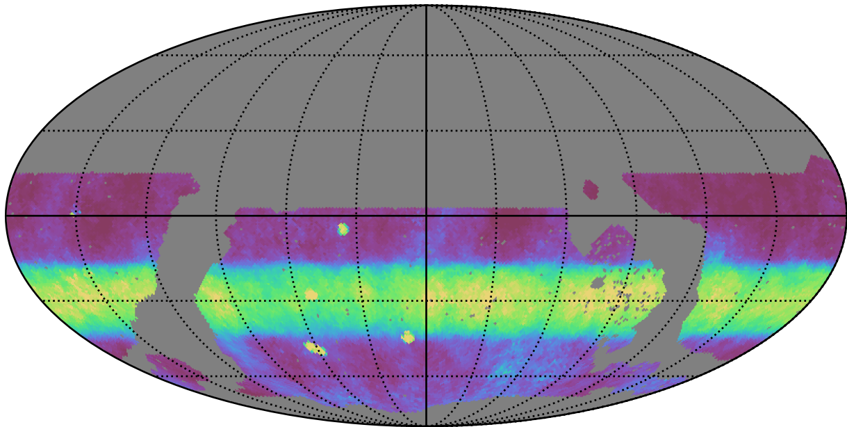
noroll_mjdp270_v3.4_10yrs WFD i band: Median normairmass
