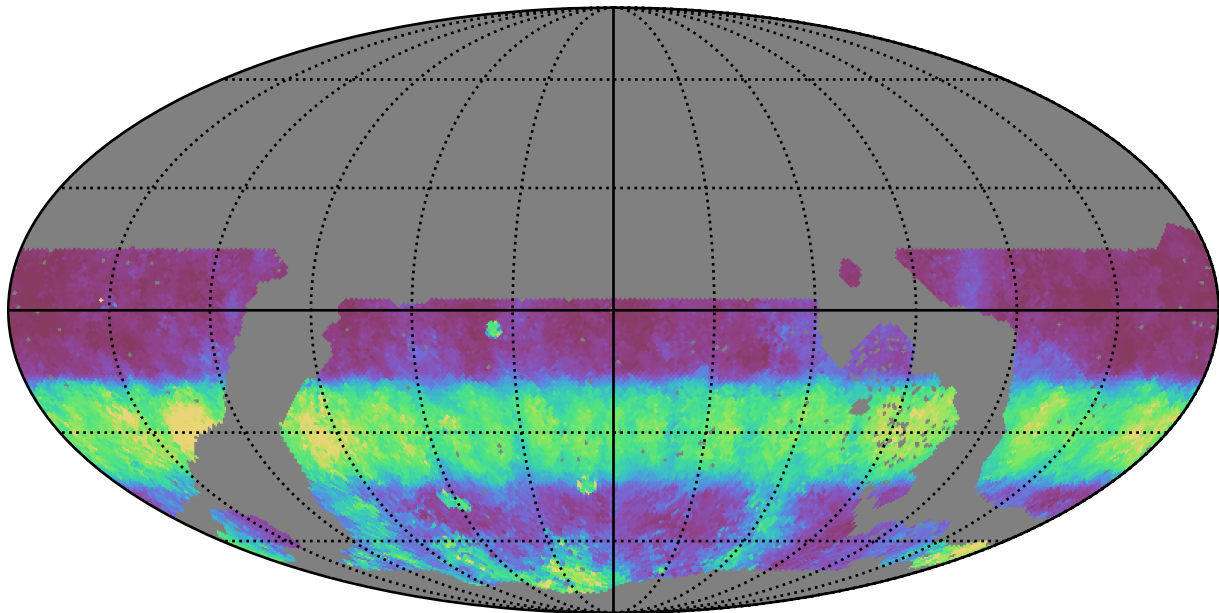
noroll_mjdp270_v3.4_10yrs WFD g band: Median normairmass
