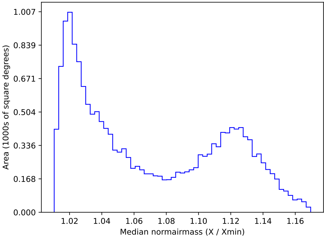
noroll_mjdp270_v3.4_10yrs WFD g band: Median normairmass
