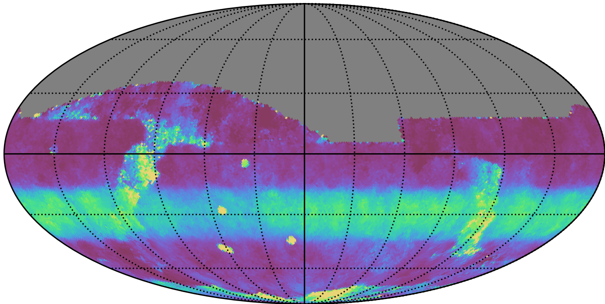
noroll_mjdp270_v3.4_10yrs All sky z band: Median normairmass
