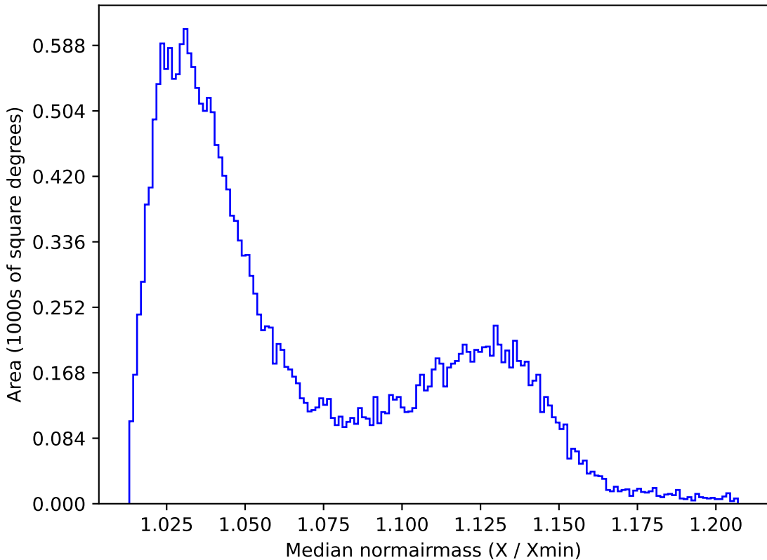
noroll_mjdp270_v3.4_10yrs All sky z band: Median normairmass
