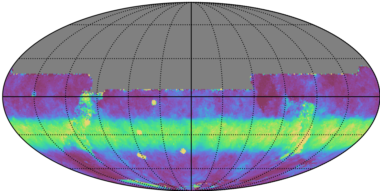
noroll_mjdp270_v3.4_10yrs All sky y band: Median normairmass
