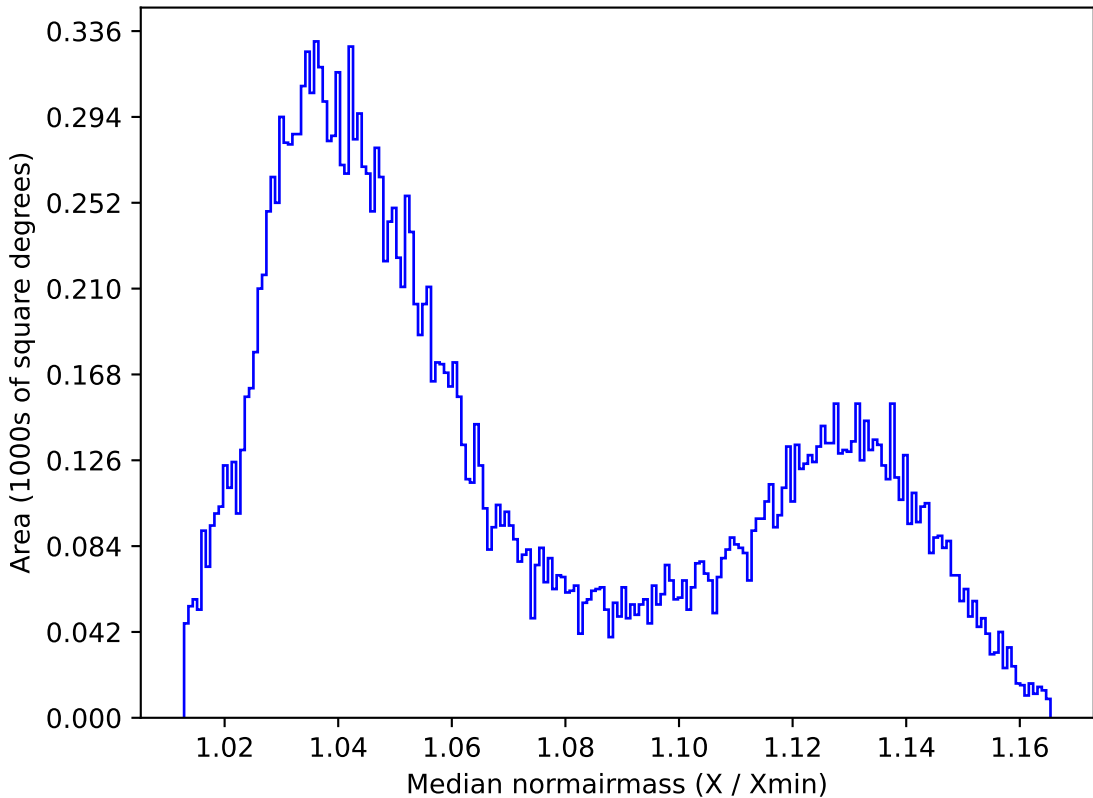
noroll_mjdp270_v3.4_10yrs All sky y band: Median normairmass
