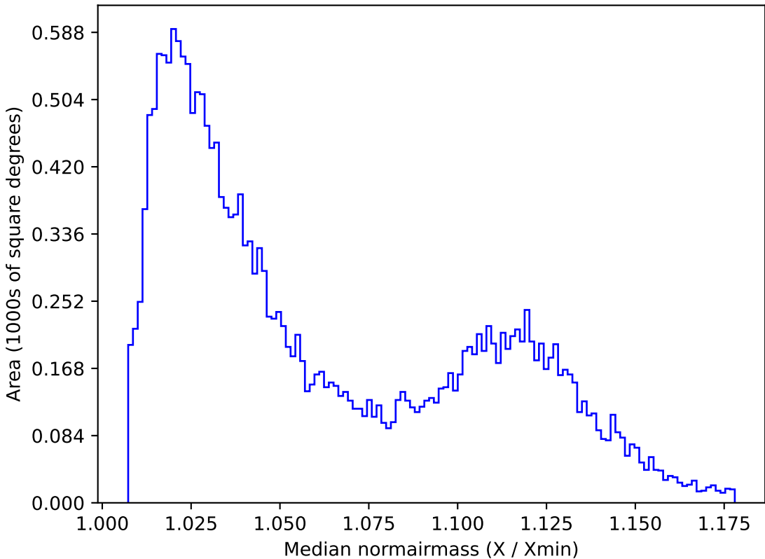
noroll_mjdp270_v3.4_10yrs All sky u band: Median normairmass
