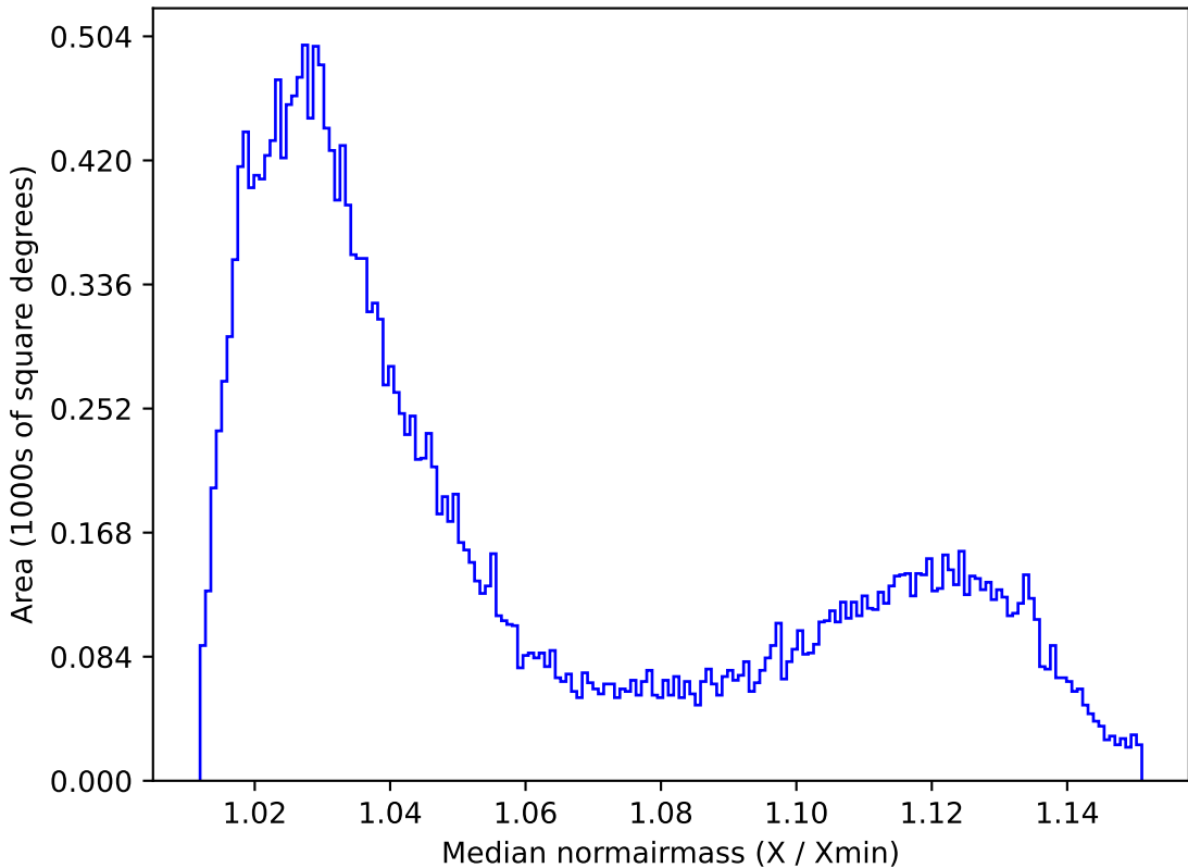
noroll_mjdp270_v3.4_10yrs All sky i band: Median normairmass
