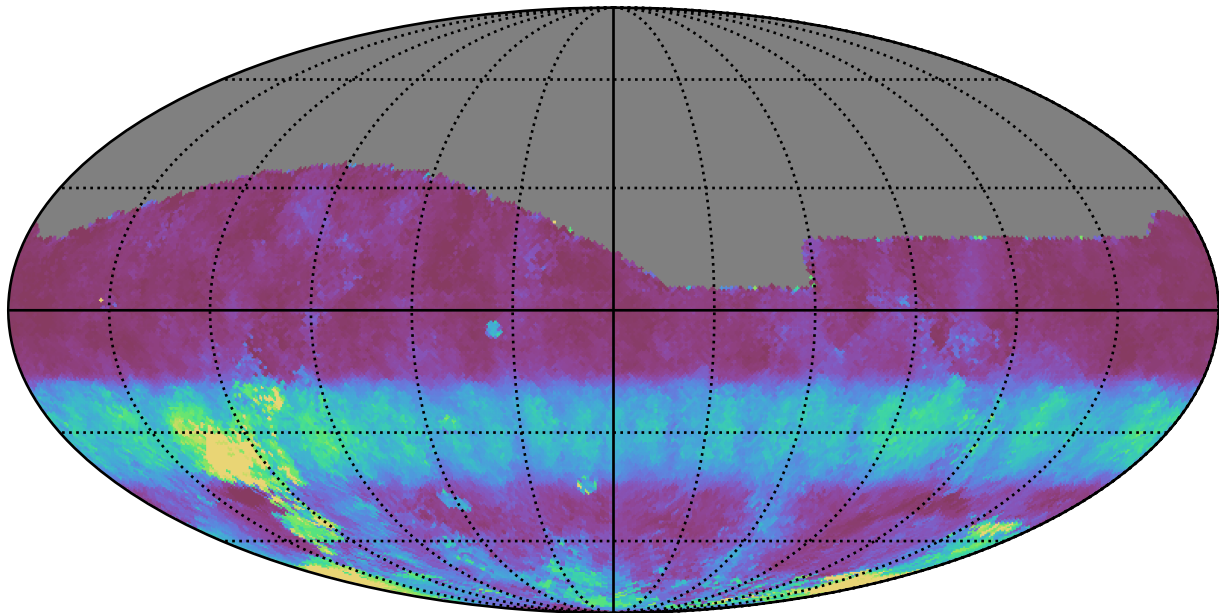
noroll_mjdp270_v3.4_10yrs All sky g band: Median normairmass
