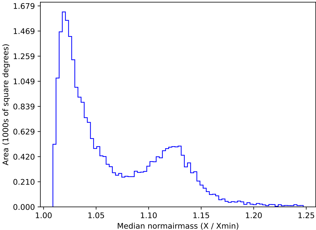
noroll_mjdp270_v3.4_10yrs All sky g band: Median normairmass
