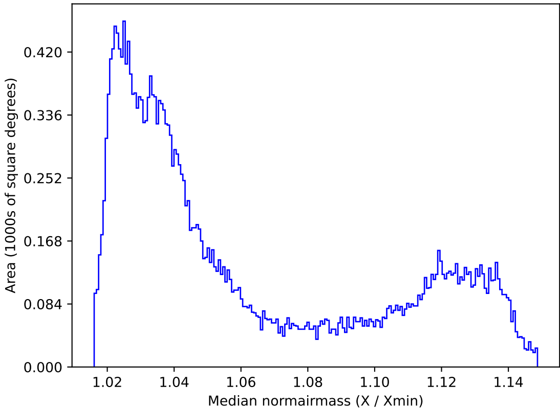
noroll_mjdp270_v3.4_10yrs All sky all bands: Median normairmass
