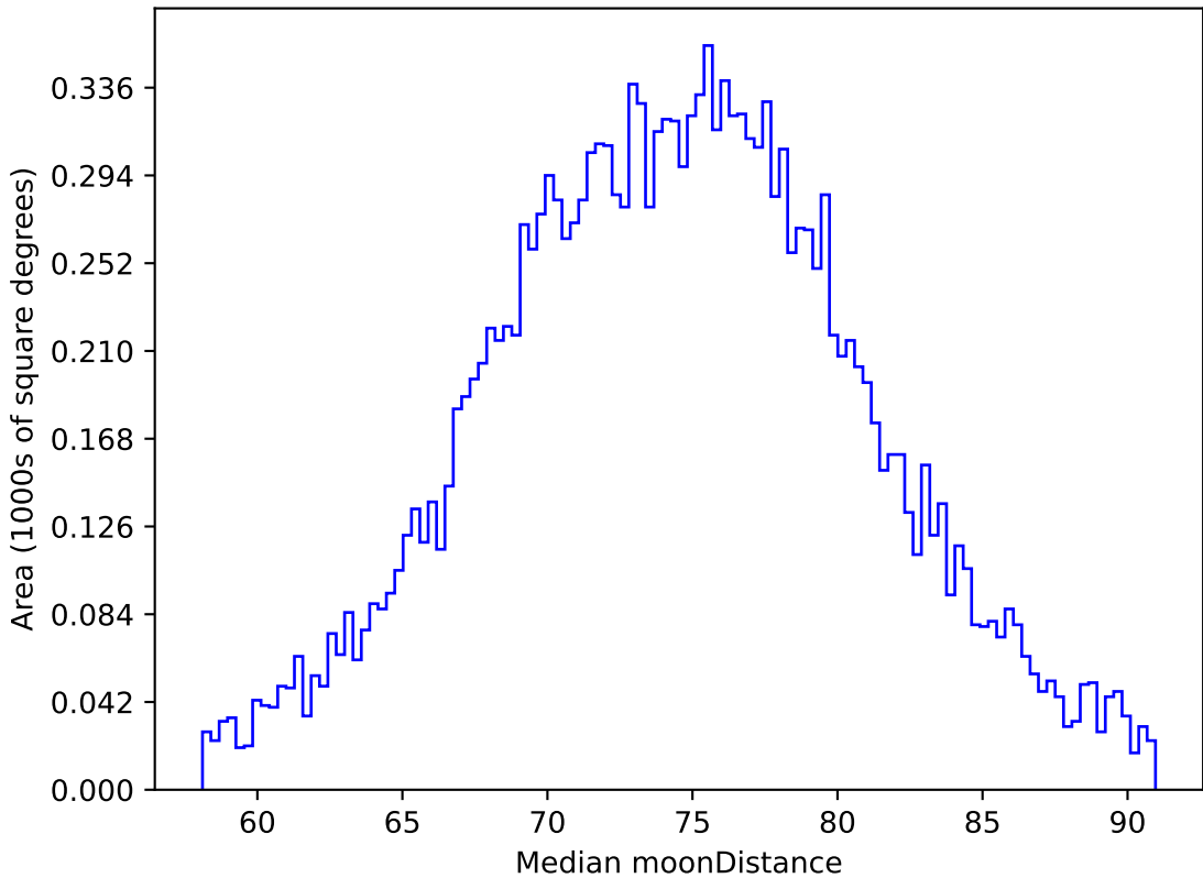
noroll_mjdp270_v3.4_10yrs WFD z band: Median moonDistance
