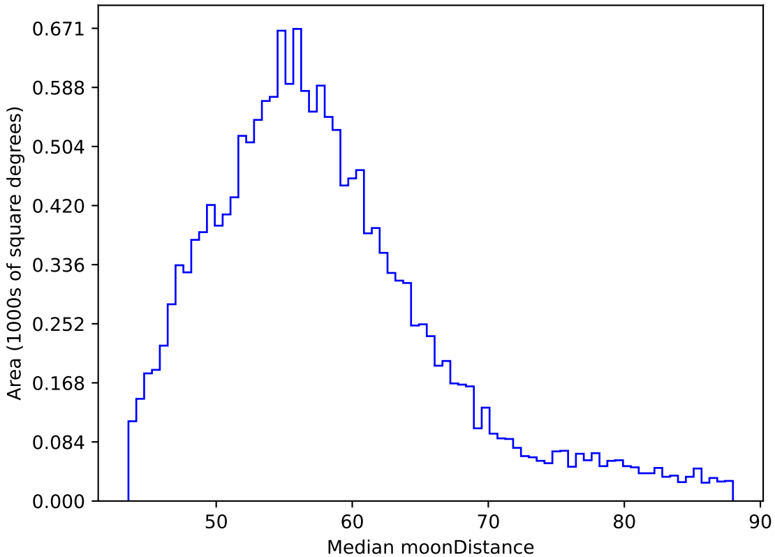
noroll_mjdp270_v3.4_10yrs WFD y band: Median moonDistance
