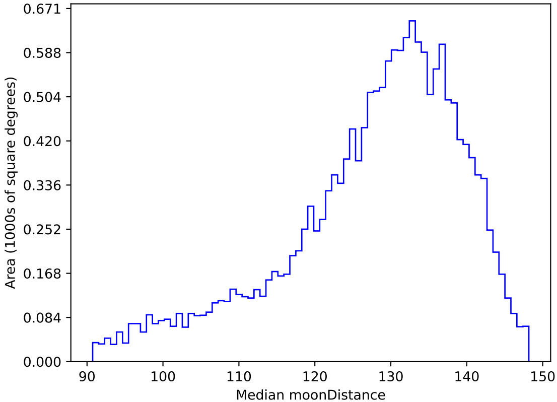
noroll_mjdp270_v3.4_10yrs WFD u band: Median moonDistance
