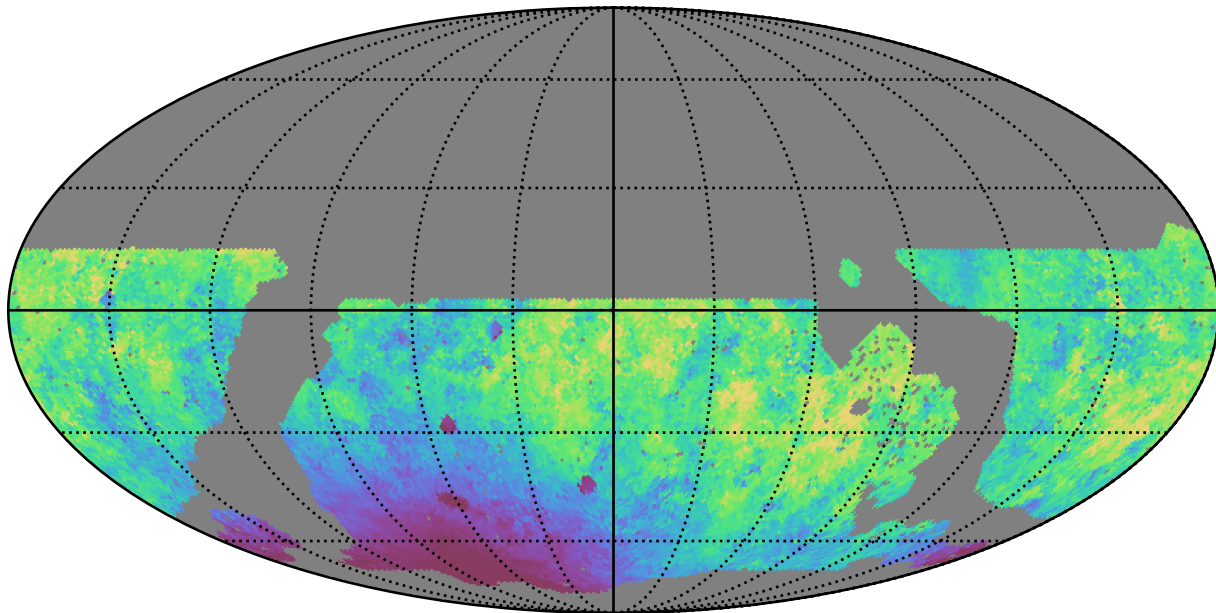
noroll_mjdp270_v3.4_10yrs WFD r band: Median moonDistance
