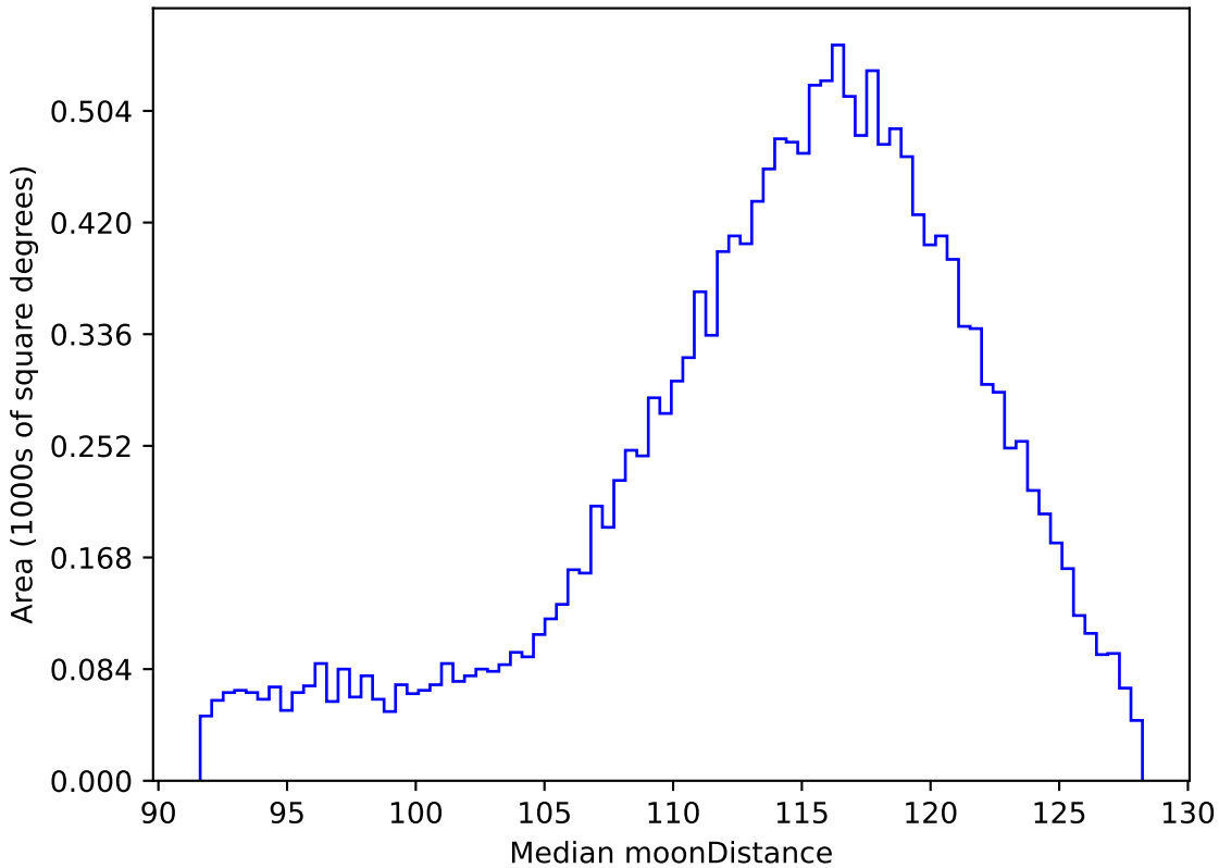
noroll_mjdp270_v3.4_10yrs WFD r band: Median moonDistance
