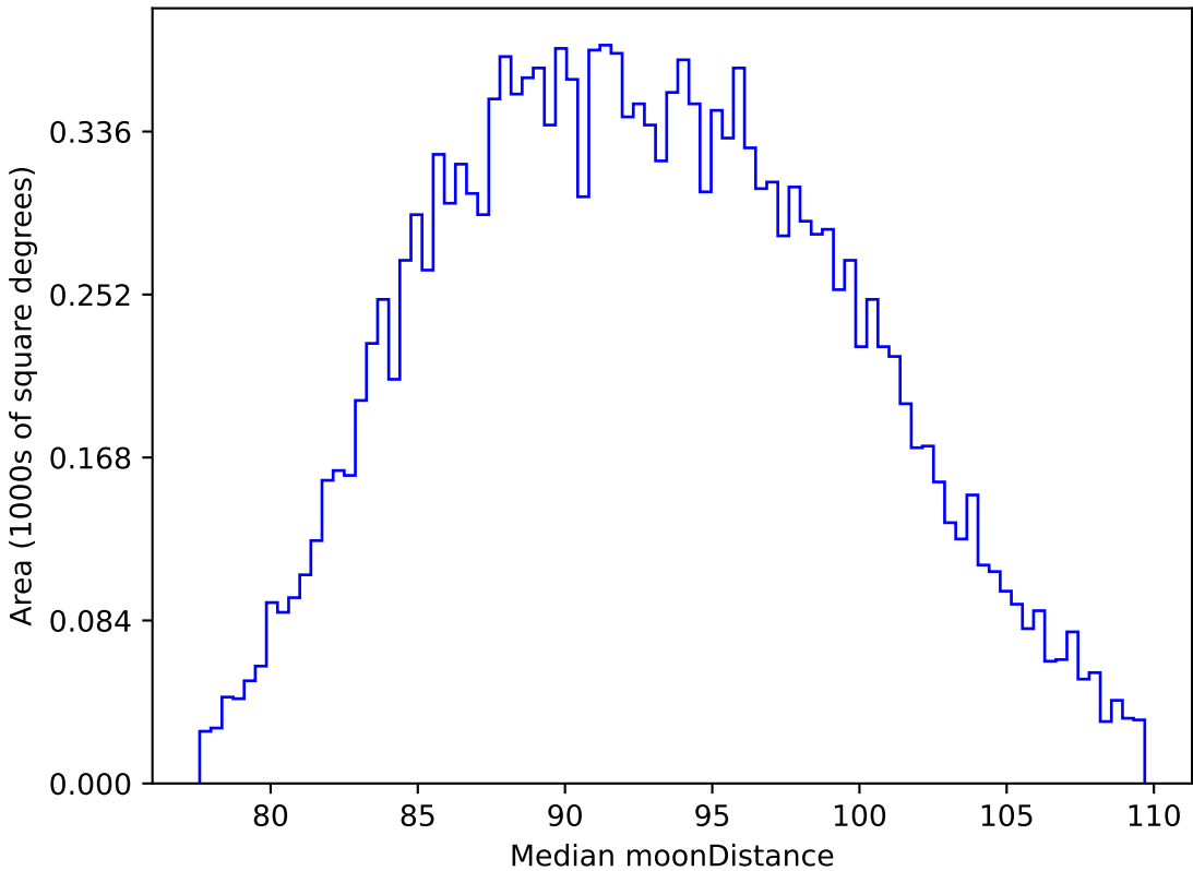
noroll_mjdp270_v3.4_10yrs WFD i band: Median moonDistance
