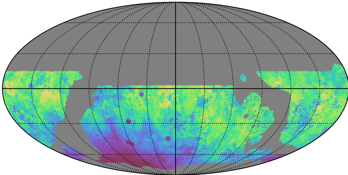
noroll_mjdp270_v3.4_10yrs WFD g band: Median moonDistance
