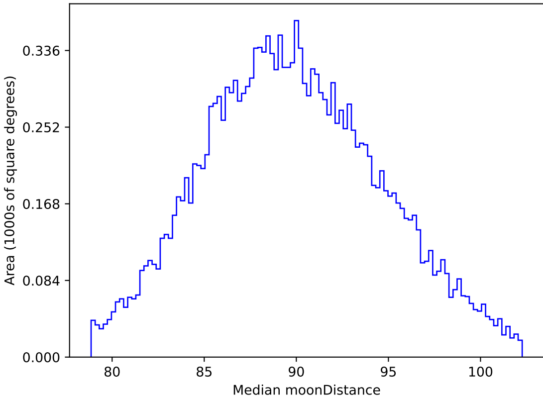
noroll_mjdp270_v3.4_10yrs WFD all bands: Median moonDistance
