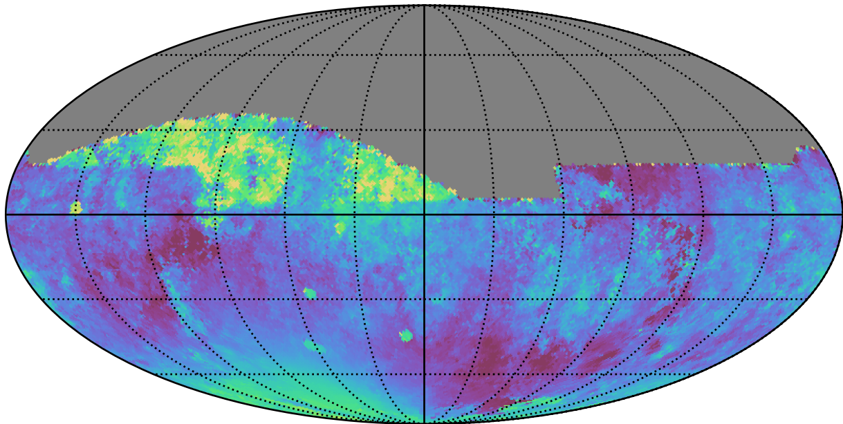
noroll_mjdp270_v3.4_10yrs All sky z band: Median moonDistance
