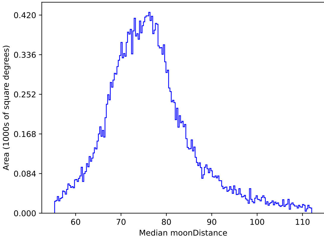
noroll_mjdp270_v3.4_10yrs All sky z band: Median moonDistance
