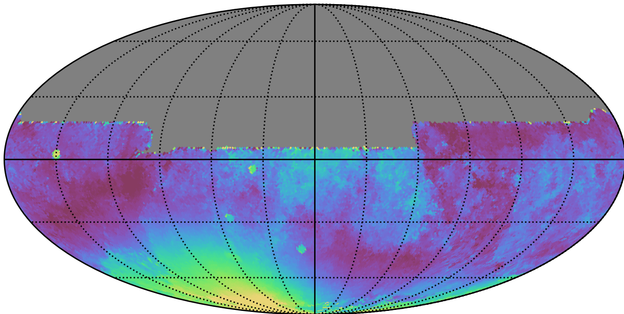
noroll_mjdp270_v3.4_10yrs All sky y band: Median moonDistance
