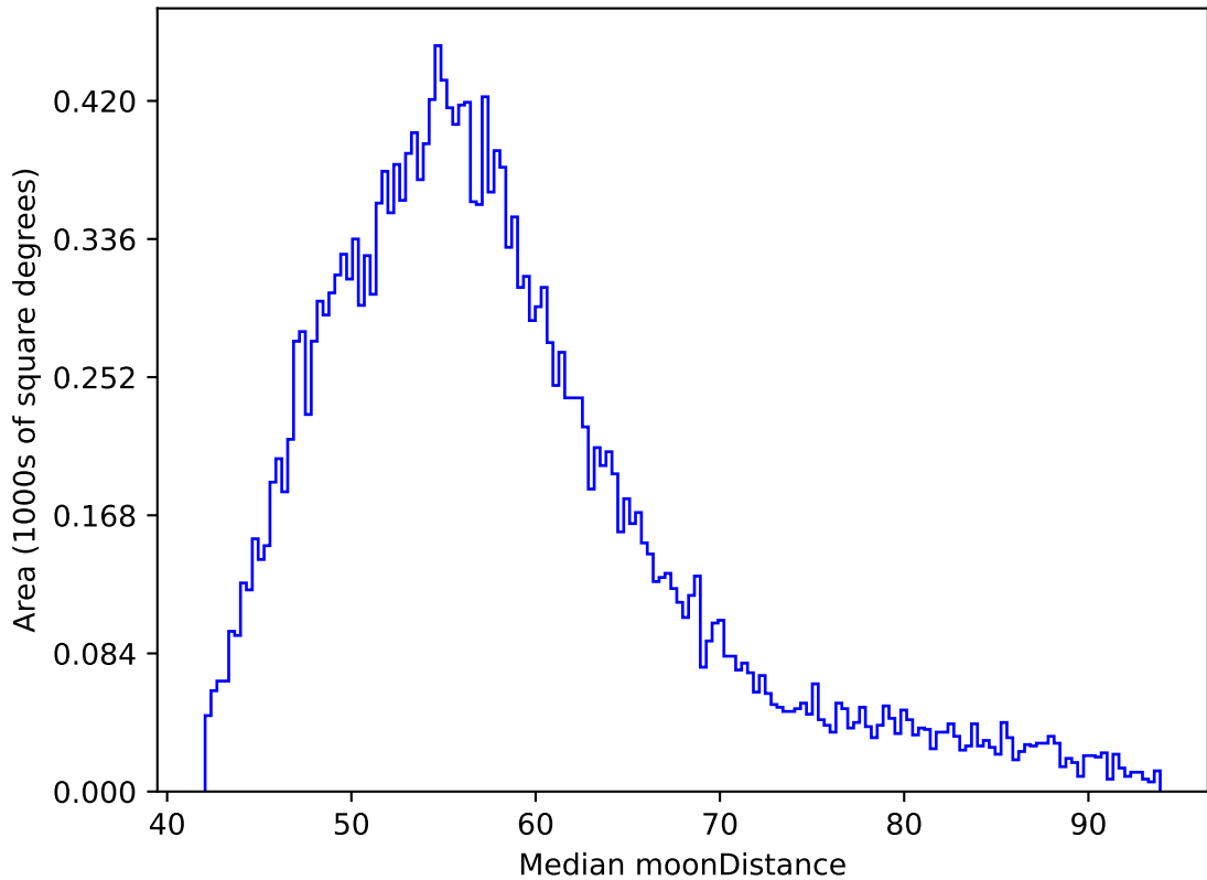
noroll_mjdp270_v3.4_10yrs All sky y band: Median moonDistance
