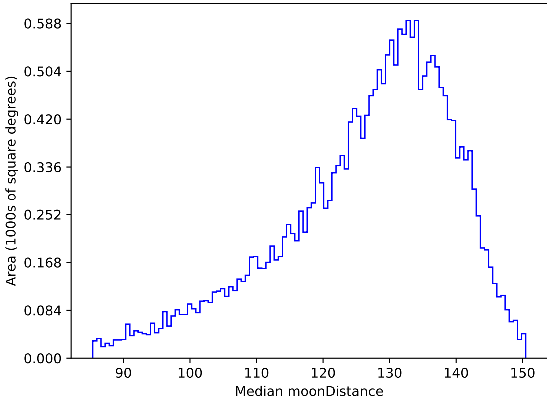
noroll_mjdp270_v3.4_10yrs All sky u band: Median moonDistance
