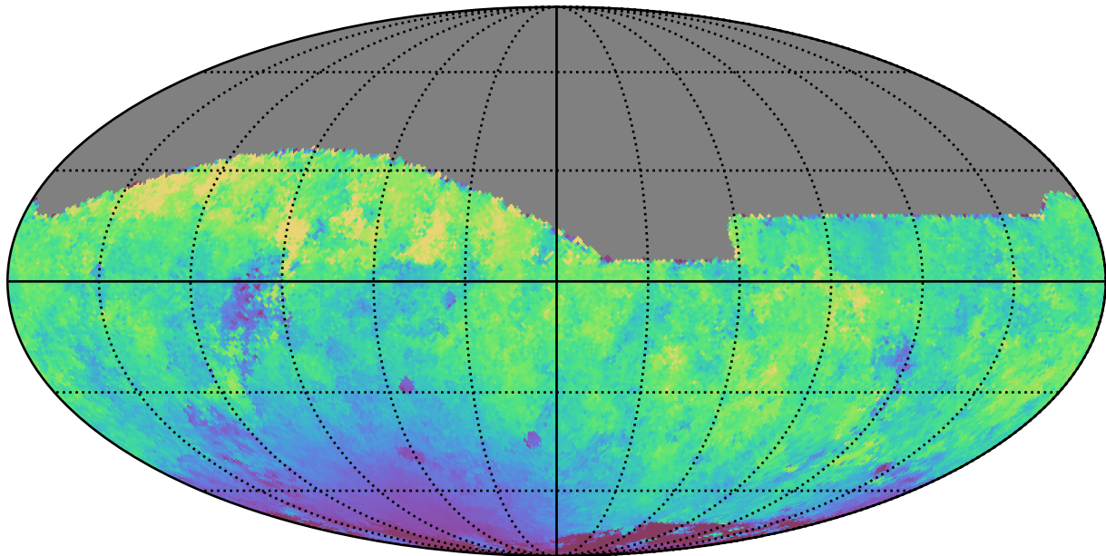
noroll_mjdp270_v3.4_10yrs All sky r band: Median moonDistance
