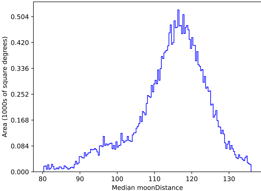
noroll_mjdp270_v3.4_10yrs All sky r band: Median moonDistance
